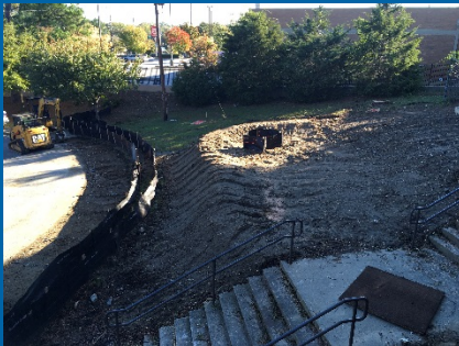
Installed New Storm Structure at Bus Loop, Silt Fence, and Site Grading
